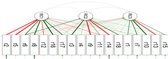
Figure 1: Structural Equation Modelling
